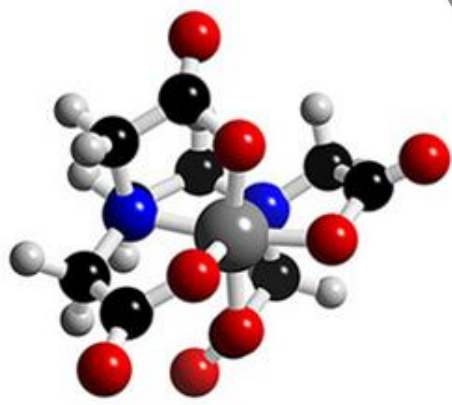
EDTA Structure Diagram of the octahedral structure of zinc EDTA forming a hexadentate chelant
